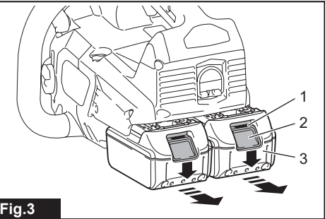
Fig.3 ► 1. Red indicator 2. Button 3. Battery cartridge
